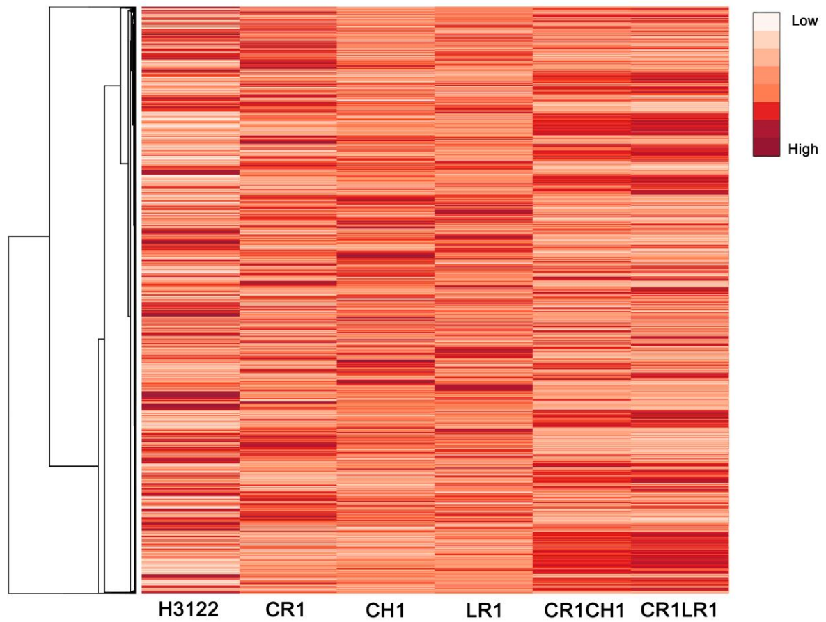
S2 Fig. The heatmap of gene expressions of whole transcriptome analysis for H3122 and anaplastic lymphoma kinase inhibitor-resistant sublines. Rows of each heat map correspond to genes sorted according to clustering (16,984 genes).
