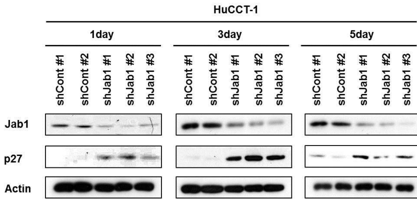
S5 Fig. Effects of Jab1 knock-down by shRNA on p27 expression. Knock-down effects of Jab1-specific shRNA were evaluated at 1 day, 3 days, and 5 days in HuCCT-1 cells.
