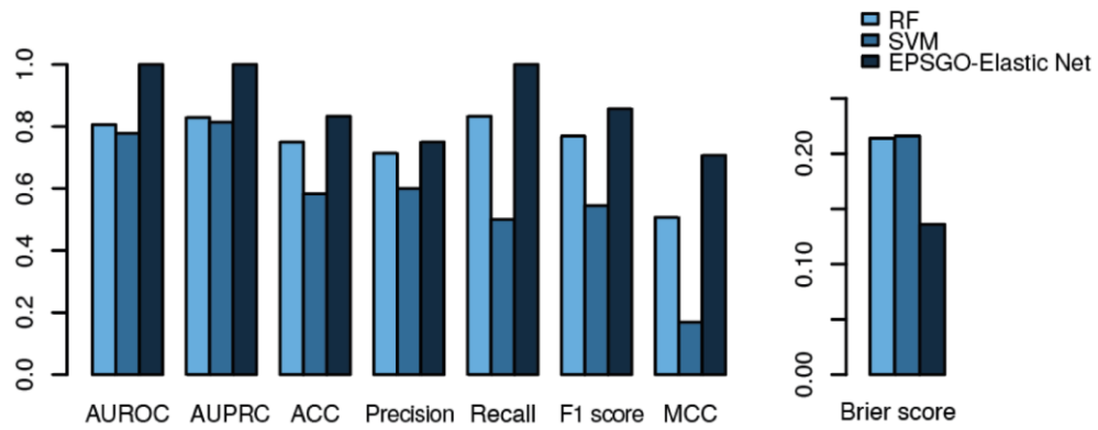
S3 Fig. Performance comparison of the three classifiers. RF, random forest; SVM, support vector machine; EPSGO, Efficient Parameter Selection via Global Optimization; AUROC, area under curve of receiver operating characteristic; AUPRC, area under the precision-recall curve; ACC, accuracy; MCC, Matthews correlation coefficient.
