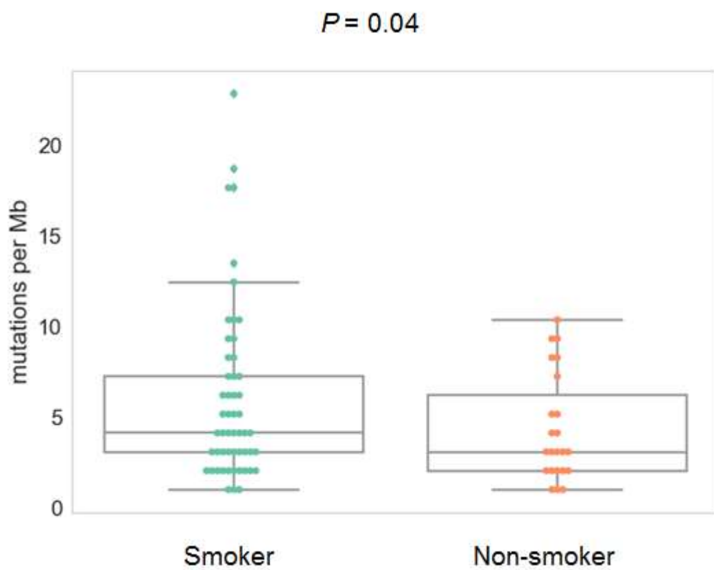
S4 Fig. Comparison of total mutational burden between smokers and non-smokers.
