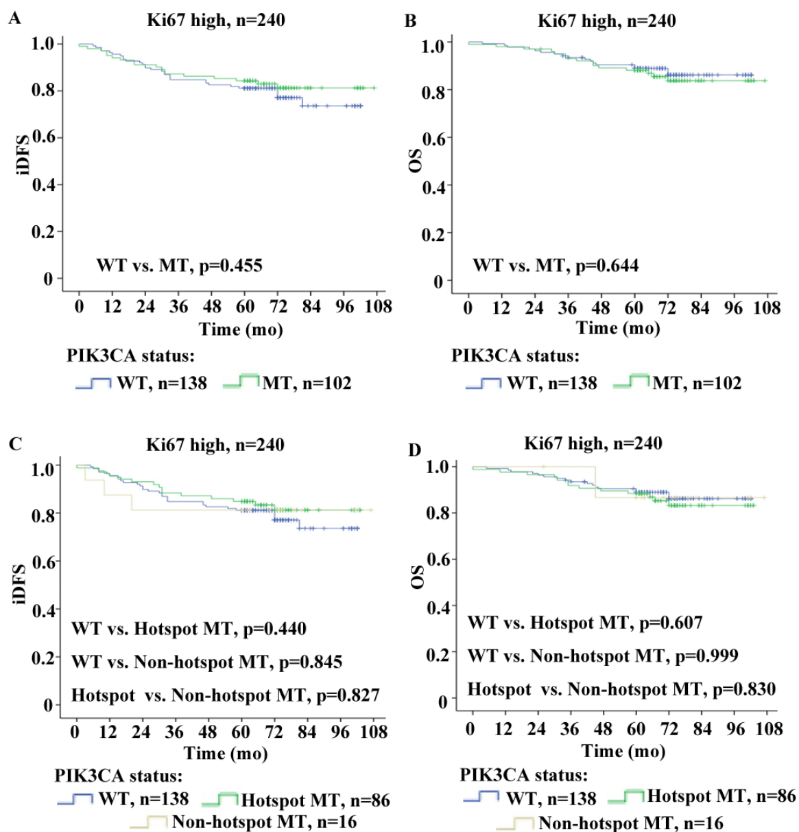
S7 Fig. Impact of PIK3CA mutations on the invasive disease-free survival (iDFS) and overall survival (OS) of 240 Ki67 high breast cancer patients with stage I-III and at least 5-year follow-up. Kaplan-Meier survival analysis; p-values calculated using a log-rank analysis. Estimated iDFS and OS by mutant status: iDFS (A) and OS (B) for patients with wild-type (WT) and mutant (MT) of PIK3CA ; iDFS (C) and OS (D) for patients with WT, hotspot MT and non-hotspot MT of PIK3CA .
