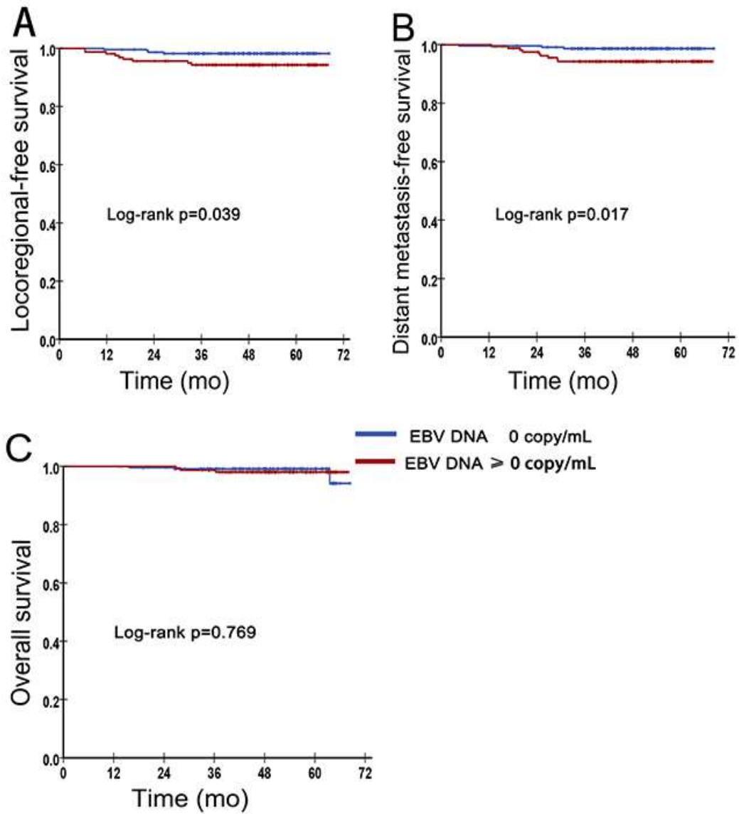
S2 Fig. Locoregional-free survival (A), distant metastasis-free survival (B), and overall survival (C) by Kaplan-Meier analysis, comparing the undetectable Epstein-Barr virus (EBV) DNA group with detectable EBV DNA group.
