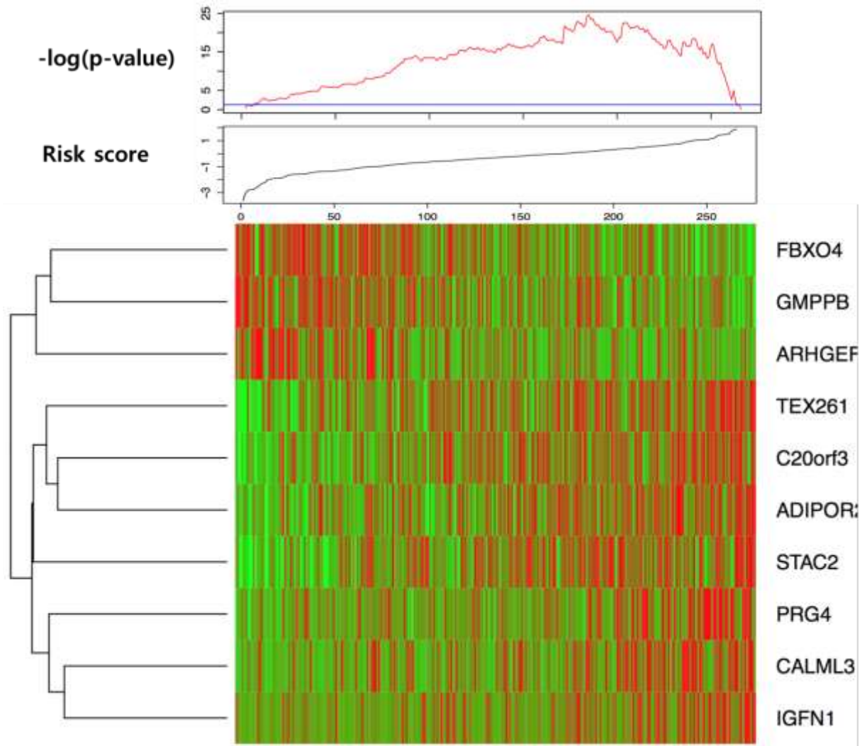
S5 Fig. Clustering by genes (mRNA) associated with survival. With each cut off value, the survival difference was significant.
