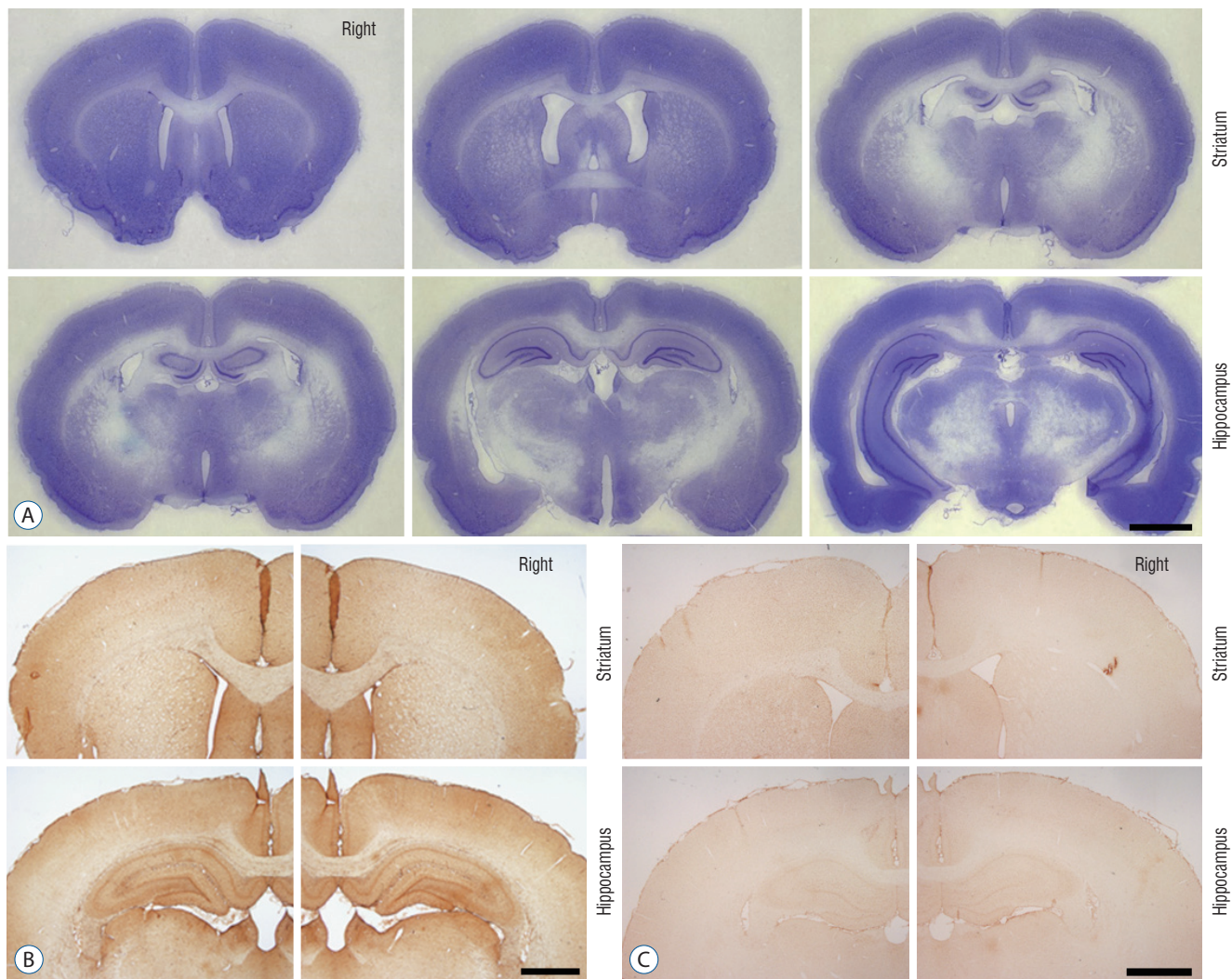
Supplementary Fig. 1. Cresyl violet (A), glial fibrillary acidic protein (B), and ionized calcium-binding adapter molecule 1 (C) staining of No. 1 rat brain of sham group on the 1st day. There are no evidence of brain damage in the right hemispheres after transient blood-brain barrier opening with mannitol, compared to the normal left hemispheres. Scale bar, 2 mm.
