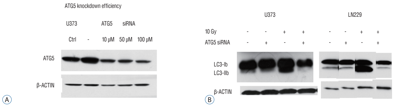
Supplementary Fig. 3. A : The efficiency of ATG5 knockdown by siRNA was confirmed by western blot. B : ATG5 knockdown decreases autophagy after irradiation in both U373 and LN229 cells. ATG5 : autophagy-related gene 5, siRNA : small interfering RNA.
