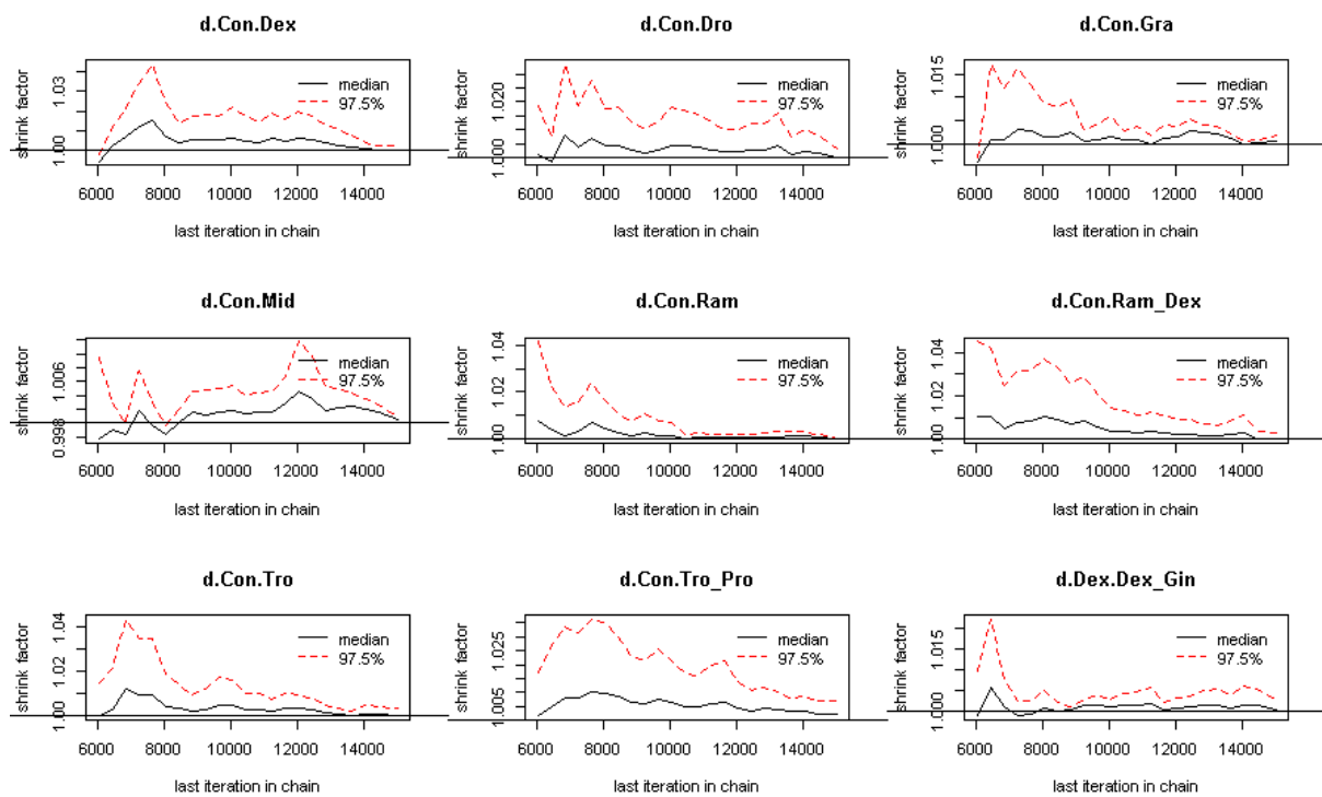
Supplementary Fig. 7. Gelman-Rubin-Brooks Plot. In Gelman-Rubin-Brooks methods, as potential scale reduction factor (PSRF) approaches 1, and the variations must be stabilized as the number of simulations increases. When PSRF approached to 1, and stabilized, it means good convergence.
