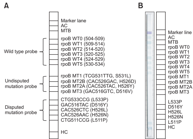
Supplementary Fig. S1. (A) A schematic illustration of each probe from the upgraded version of the MolecuTech REBA MTB-MDR Kit. (B) Detection of the CTG511CCG (L511P) disputed rpoB mutation using the upgraded version of the MolecuTech REBA MTB-MDR Kit.
