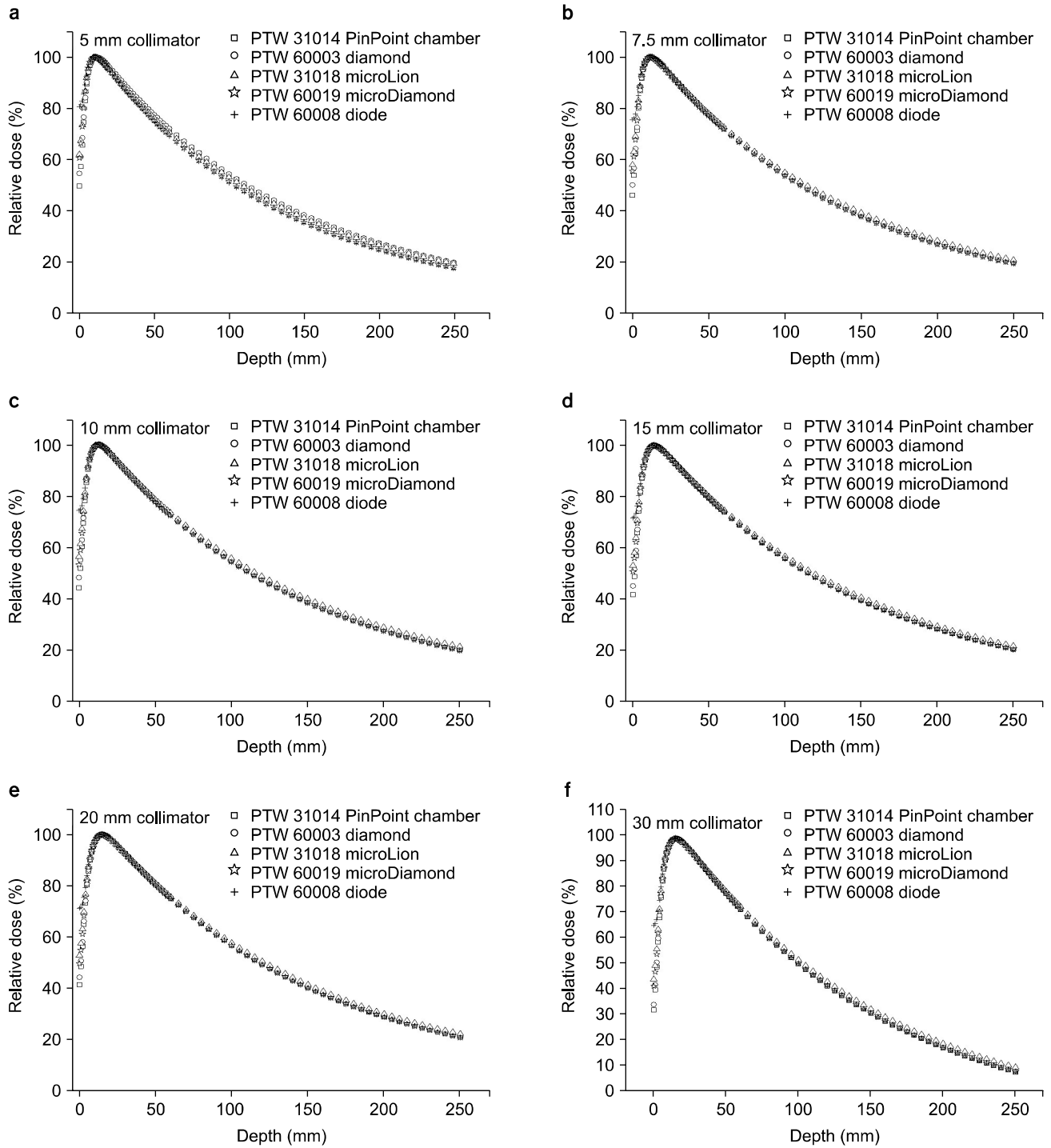
Fig. 6. Depth-dose curves as measured with the each detectors at (a) 5 mm, (b) 7.5 mm, (c) 10 mm, (d) 15 mm, (e) 20 mm, and (f) 30 mm collimator, respectively. All depth-dose curves are taken from water surface to 25 cm depth at SSD 100 cm.
