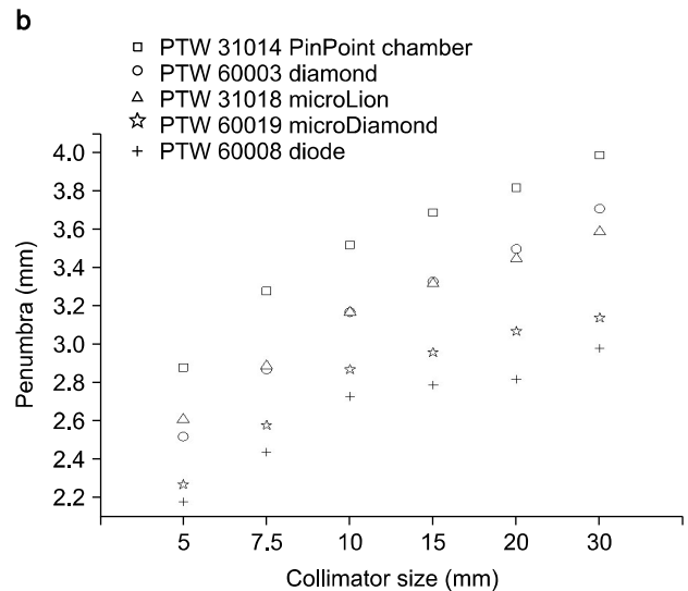
Fig. 8. (a) The lateral dose profiles measured with the each detectors at 6 collimator size, respectively. All profiles are taken at 5 cm depth water at 80 cm SAD. (b) 80%~20% penumbra values derived from the lateral beam profiles.
