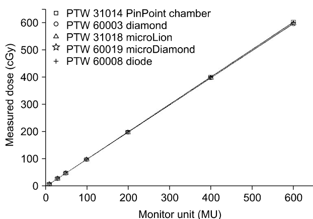
Fig. 3. The comparison of dose linearity for each detectors response were measured from 10 to 600 MU in 10 \times 10 cm 2 field with respect to the dose rate of 300 MU/min. Linear fit is plotted with solid line.
