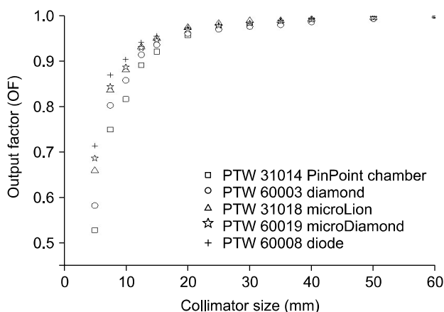
Fig. 5. The comparison of output factors for each detectors were measured in diameter from 0.5 \times 0.5 \text{ cm}^2 to 6 \times 6 \text{ cm}^2 with CyberKnife system.
