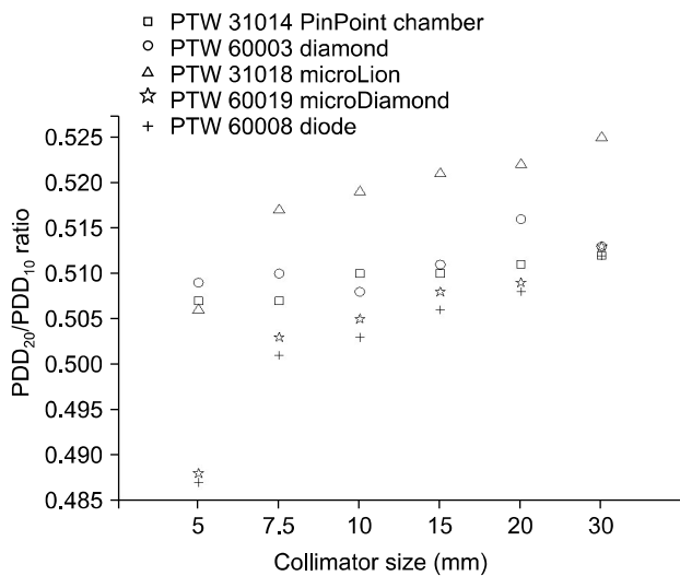
Fig. 7. PDD_{20}/PDD_{10} ratio values derived from depth-dose curves.
