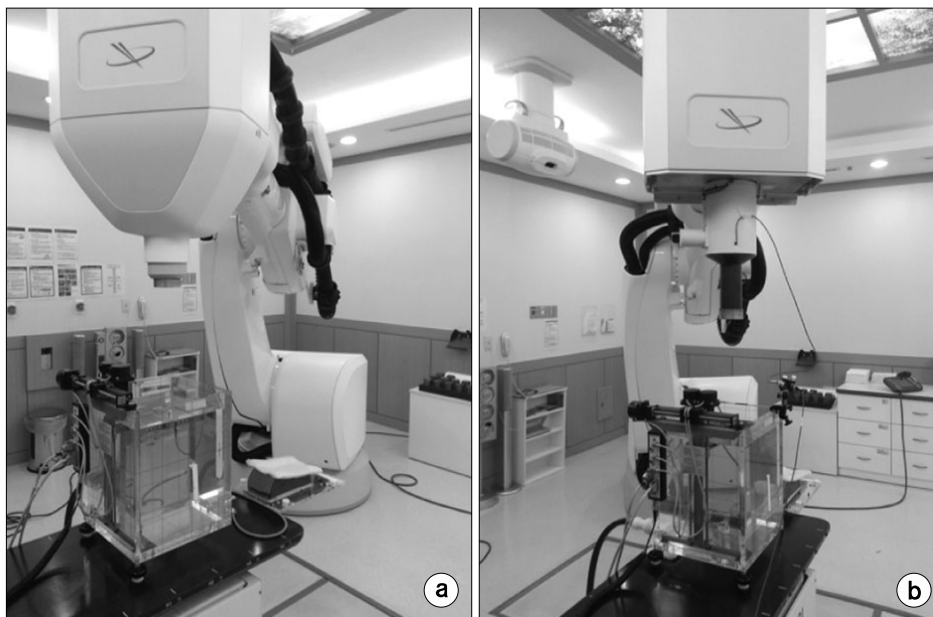
Fig. 2. Photographs depicting the experimental setup of cyberknife and water phantom. The source-detector distance of 80 cm at 1.5 \text{ g/cm}^2 , 5 cm \text{g/cm}^2 depth for measurement of (a) OF and (b) OCR, respectively. The measurement of dosimetric parameters with (b) PDD was scanned at SSD = 80 cm, from water surface to 25 cm depth.
