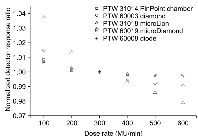
Fig. 4. The comparison of dose rate dependence for each detectors response were measured from 100 to 600 MU/min in 10 \times 10 cm 2 field at delivered dose 100 MU. Detector response at dose rate 300 MU/min was normalized to 1.
