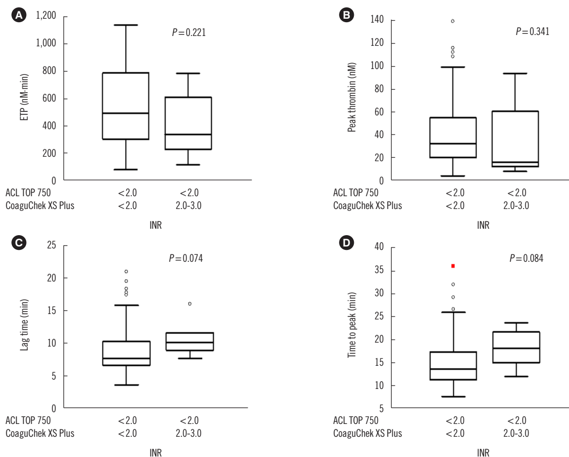
Supplemental Data Fig. S1. Differences in (A) ETP, (B) peak thrombin, (C) lag time, and (D) time to peak between the accord group (INR <2.0 by both CoaguChek XS Plus and ACL TOP 750) and discrepancy group 2 (2.0 ≤ INR ≤ 3.0 by CoaguChek XS Plus and INR <2.0 by ACL TOP 750). The red symbol in Fig. S1D indicates a value higher than the upper outer fence, which is calculated by adding three times the interquartile range to the 3rd quartile.
