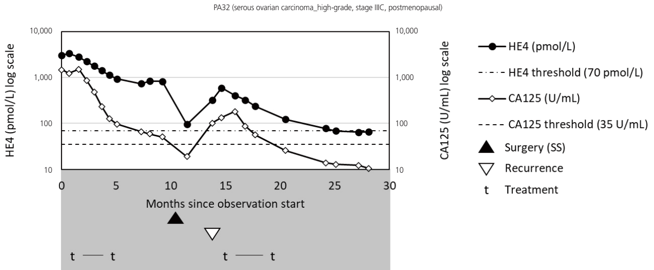
Supplementary Fig. 26. Graphical representation of a patient with recurrence (PA32). The HE4 value is displayed on the log scale on the left vertical axis, and the CA125 value is displayed on the log scale on the right vertical axis. HE4, human epididymis protein 4; CA125, cancer antigen 125; SS, suboptimal surgery.
