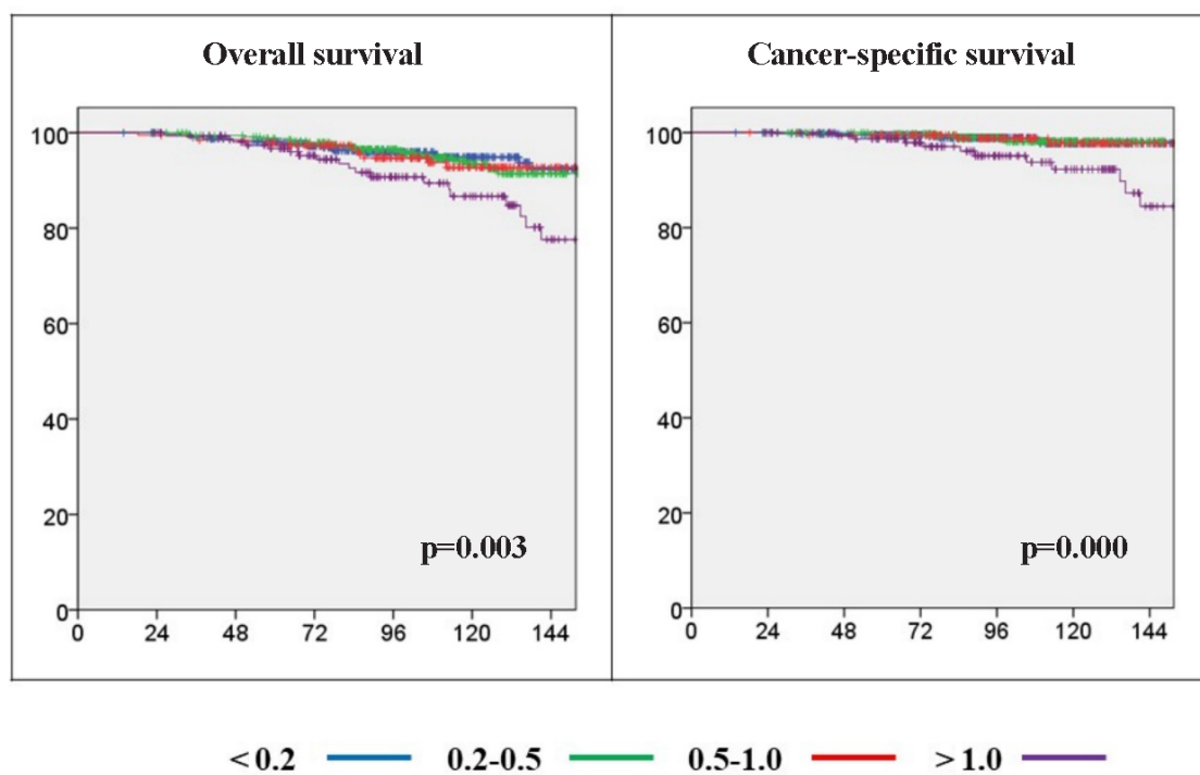
S2 Fig. Overall survival and cancer-specific survival from the day of RP according to pre-PORT PSA level. RP, radical prostatectomy; PORT, postoperative radiotherapy; PSA, prostate-specific antigen.
