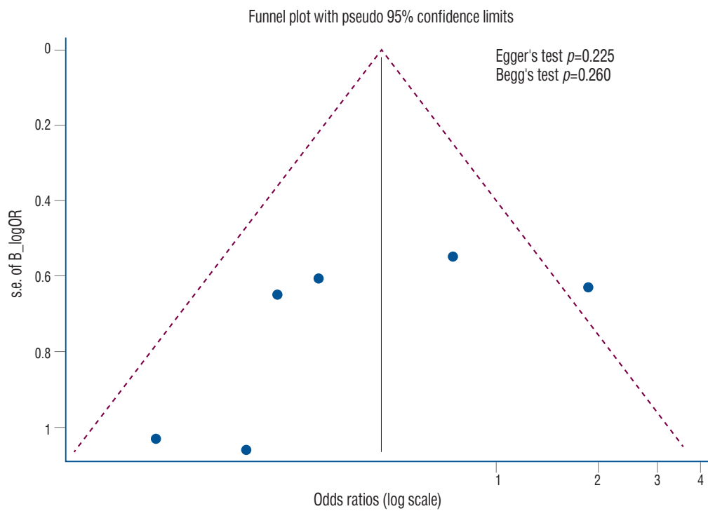
Supplementary Fig. 1. Funnel plots for evaluating publication bias. Funnel plot revealed that there was no evidence for publication bias of across the direct comparisons between arachnoid plasty group and control in patients underwent clipping surgery for unruptured intracranial aneurysm. s.e. : standard error.
